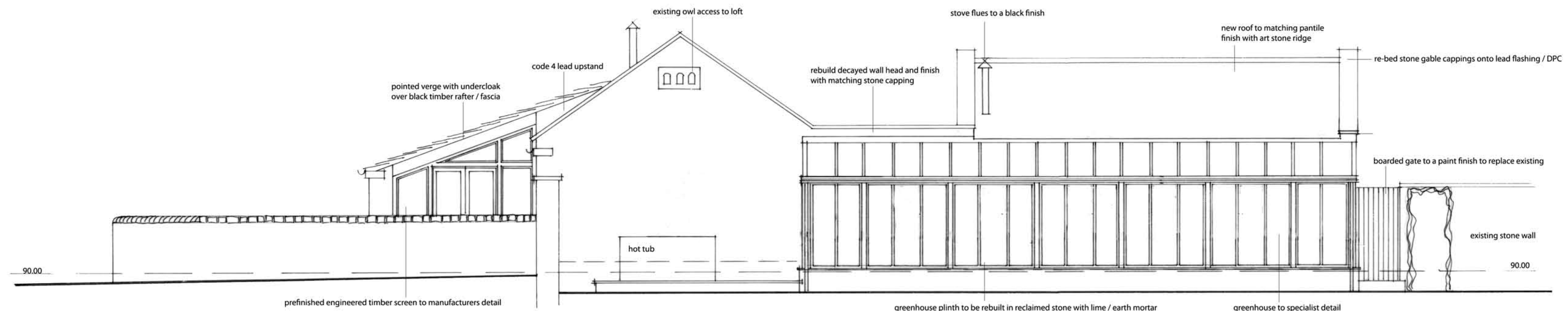
South Elevation
