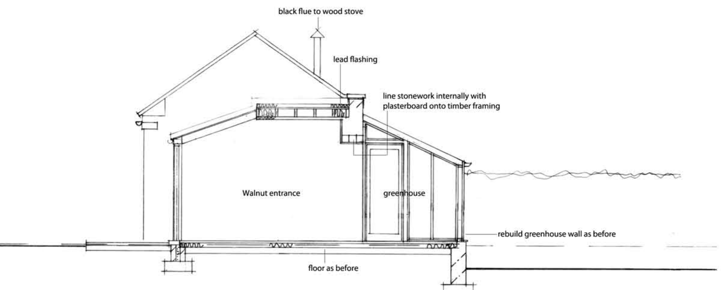
Section D / D
