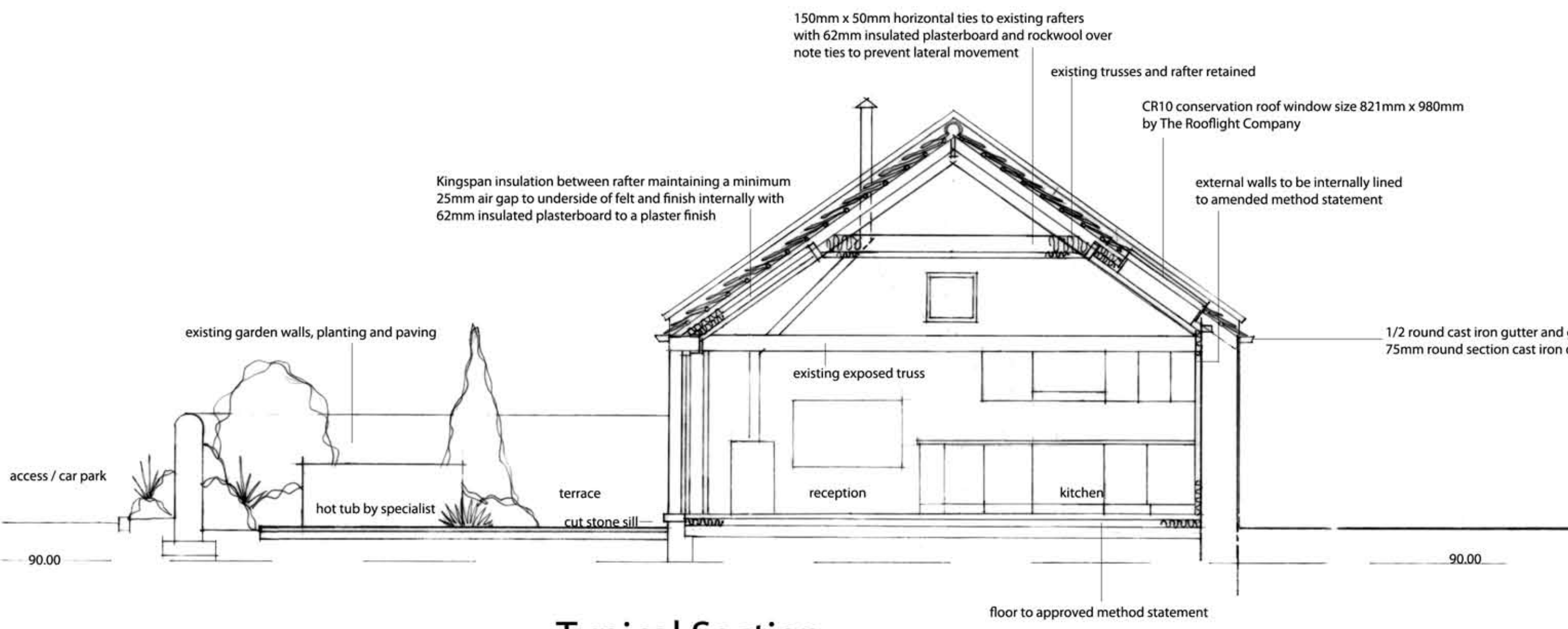
Typical Section
