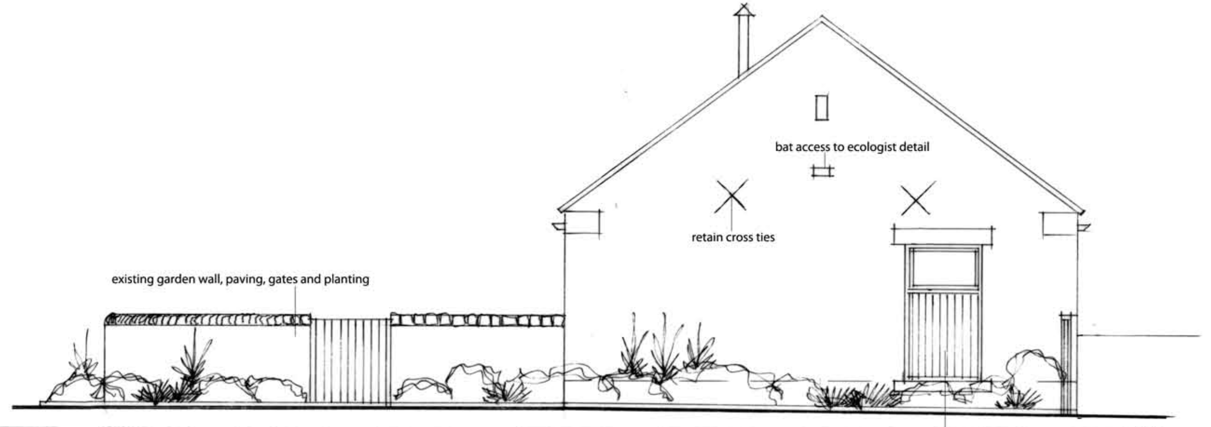
West Elevation
