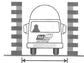
The tanker which delivers is 2.6m (8'6") wide
