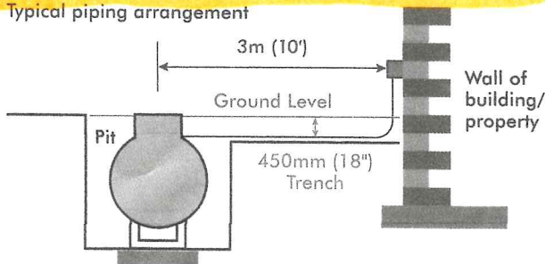
Typical piping arrangement
