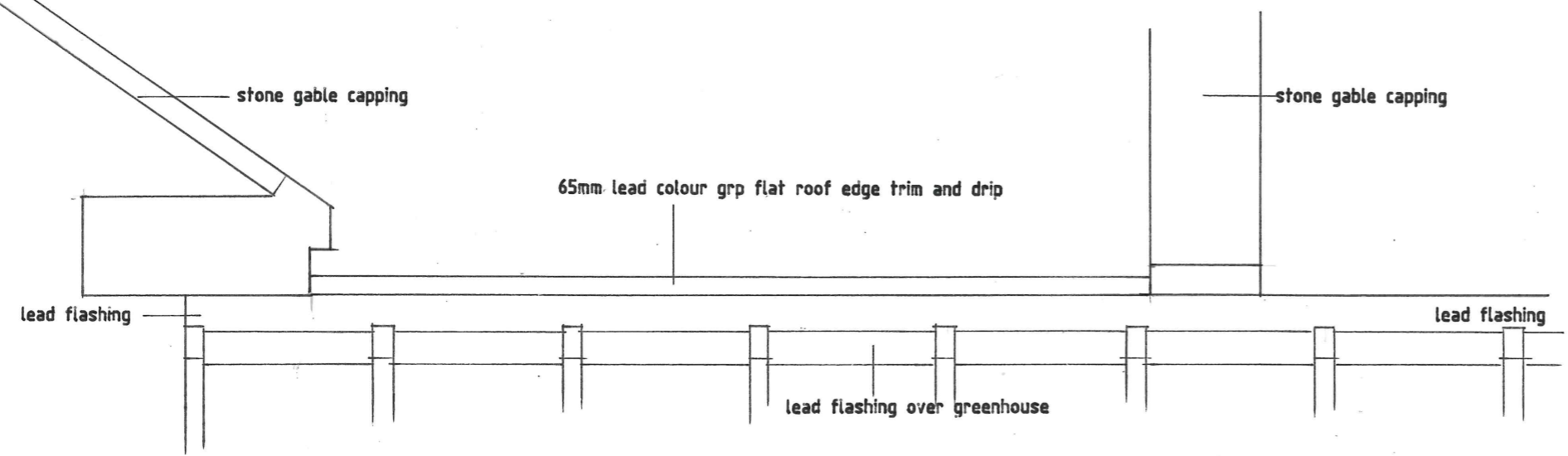
Elevation Detail
