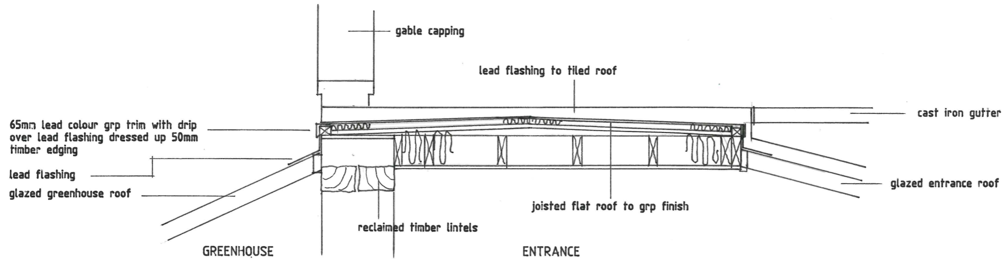
Section Detail
