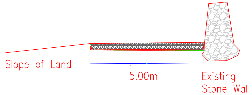
Cross section of track adjacent to existing walls.
