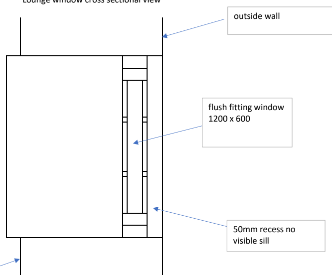
Lounge window cross sectional view
