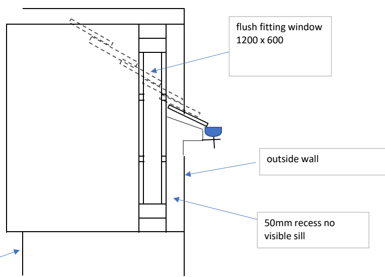
Bedroom 2 window cross sectional view
