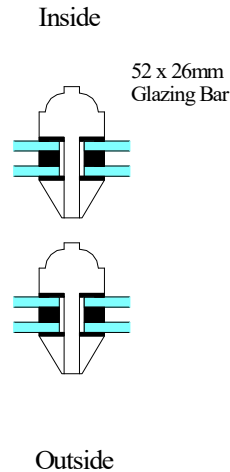
Horizontal Section Through
