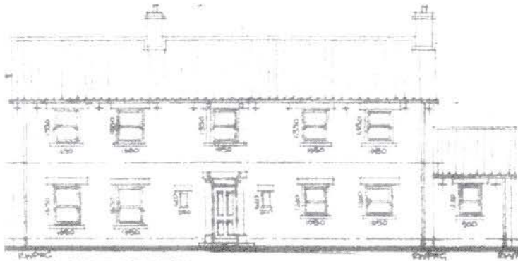
SOUTH FRONT ELEVATION
