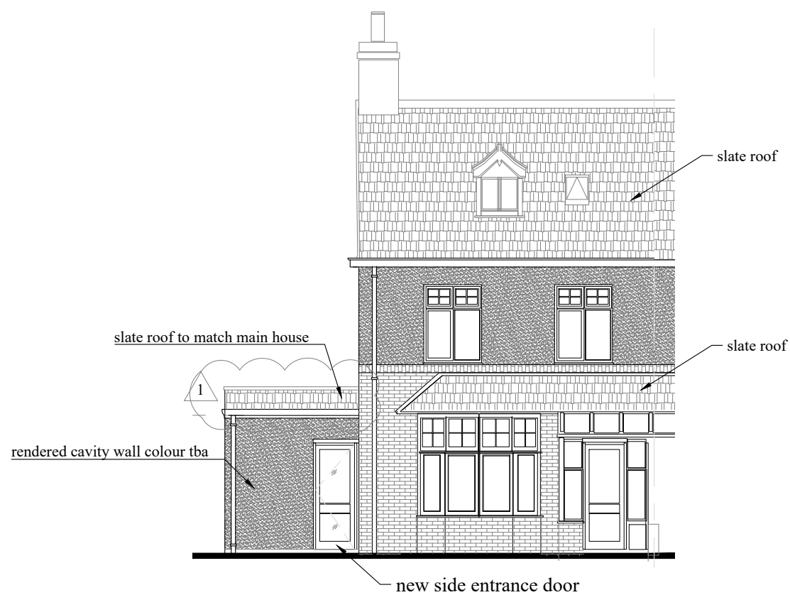
EAST ELEVATION
