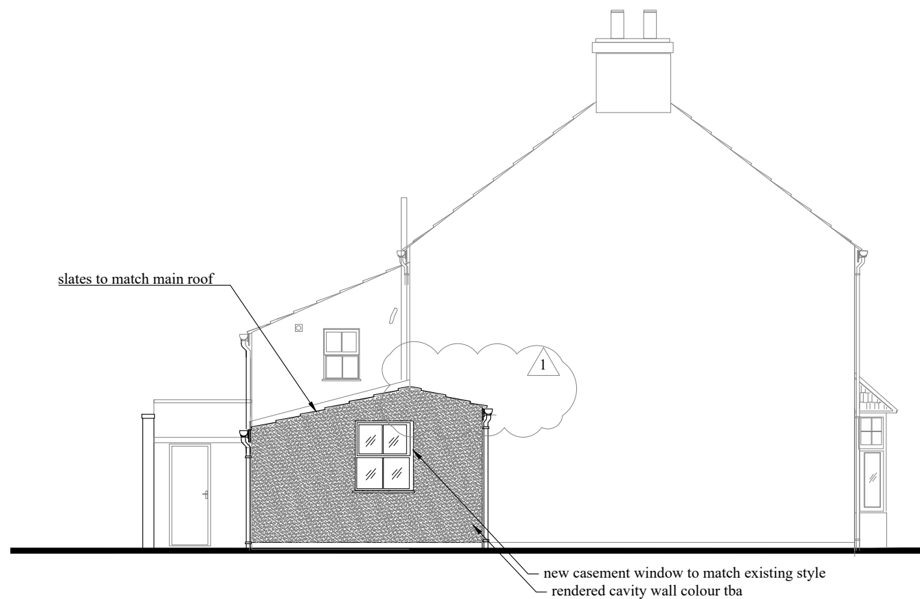
SOUTH ELEVATION
