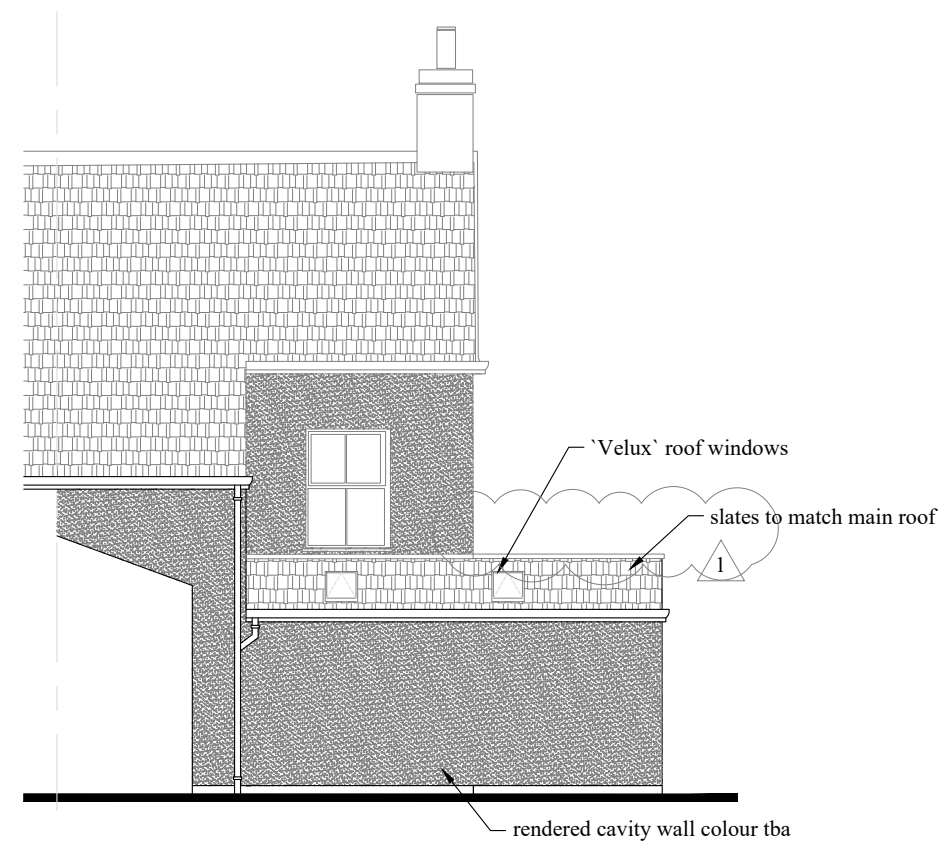
WEST ELEVATION
