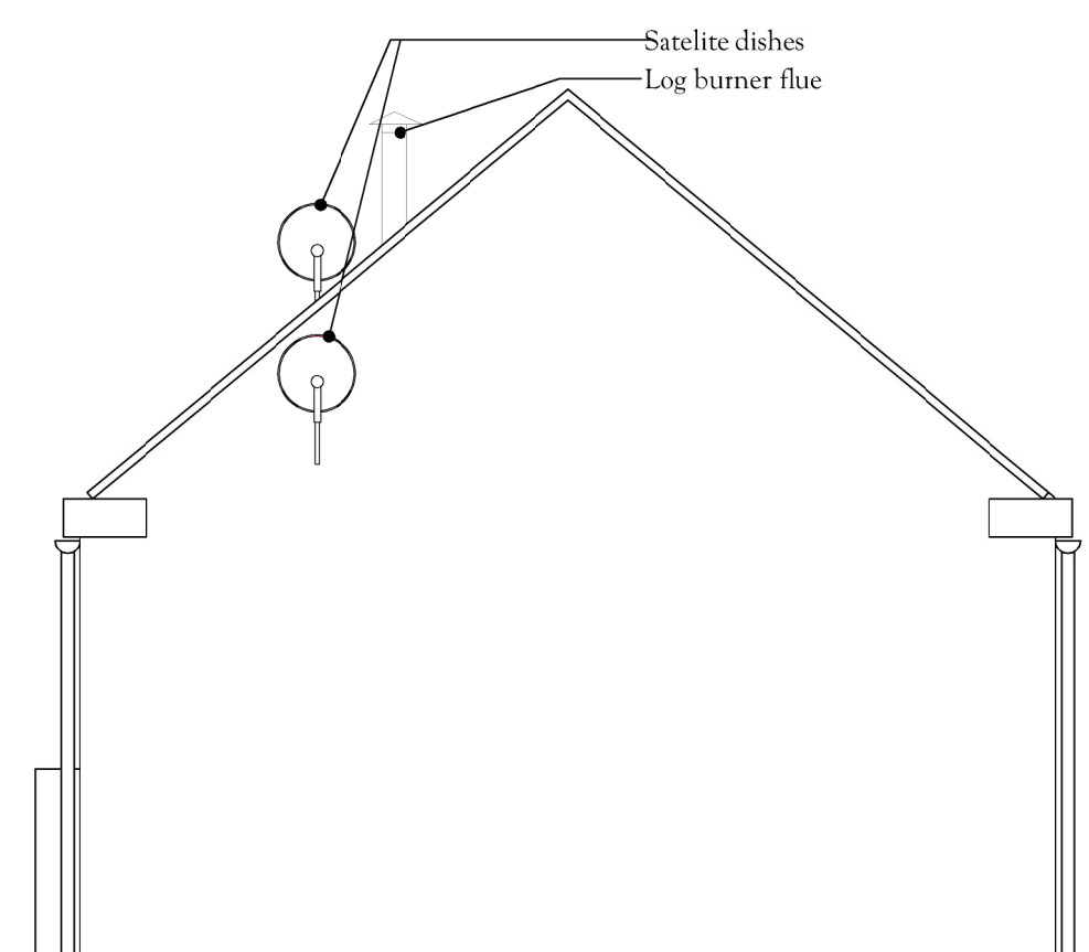
South West Elevation Proposed Elevations - 1:50
