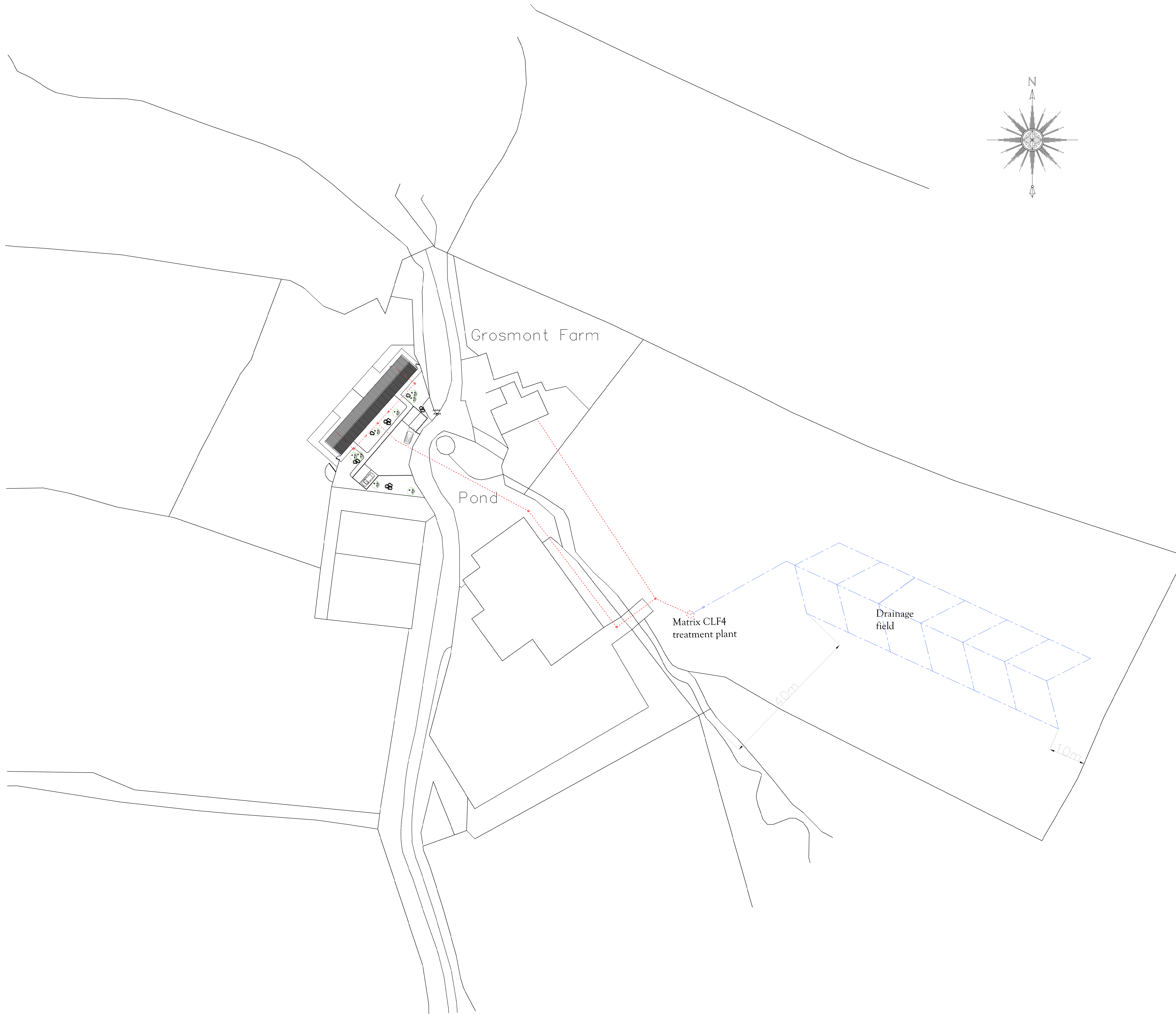
Drainage Field Plan - 1:500
