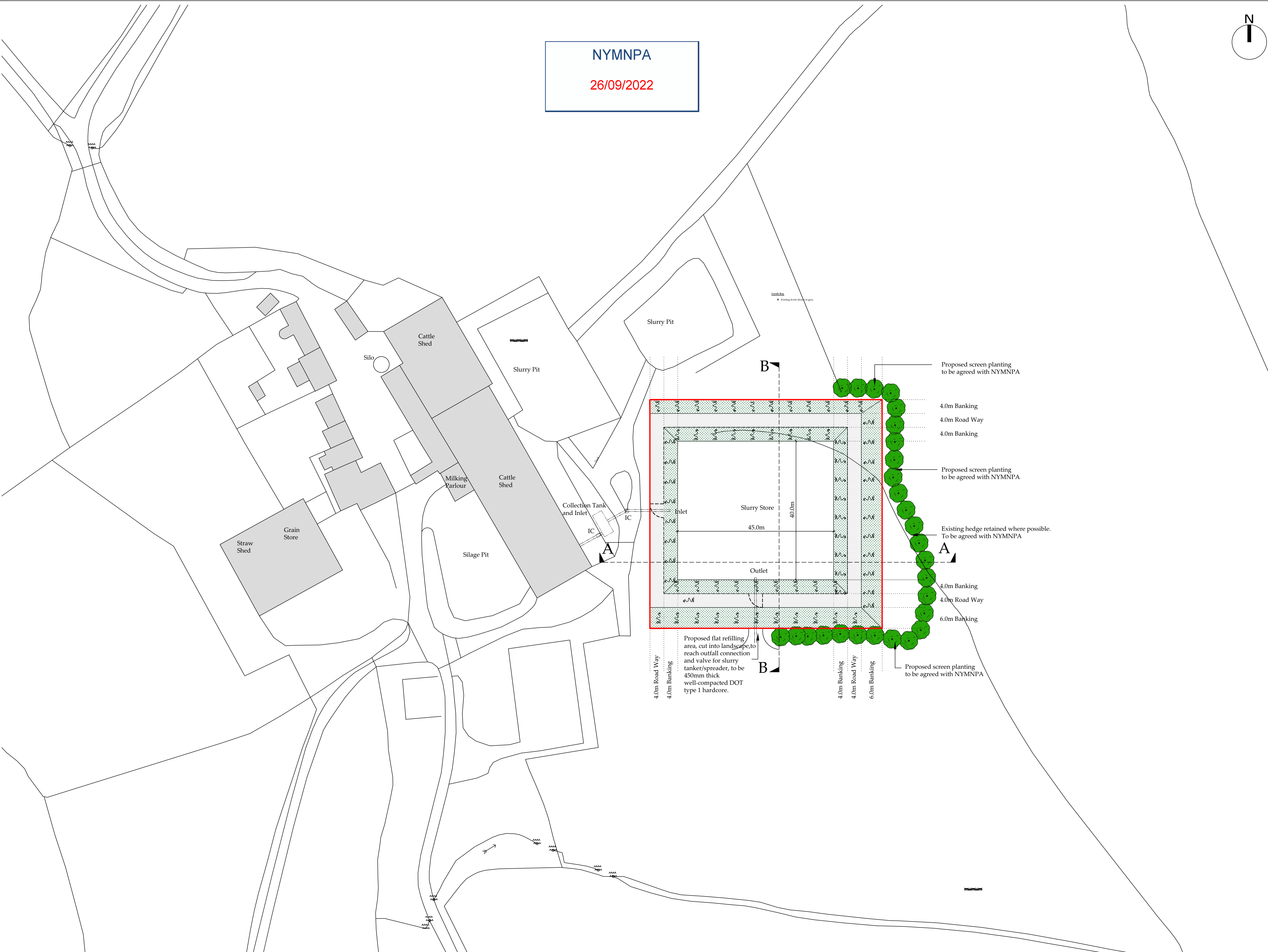
Block Plan Scale 1:200
