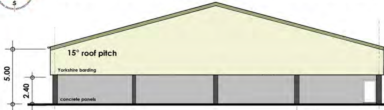
NORTH ELEVATION
