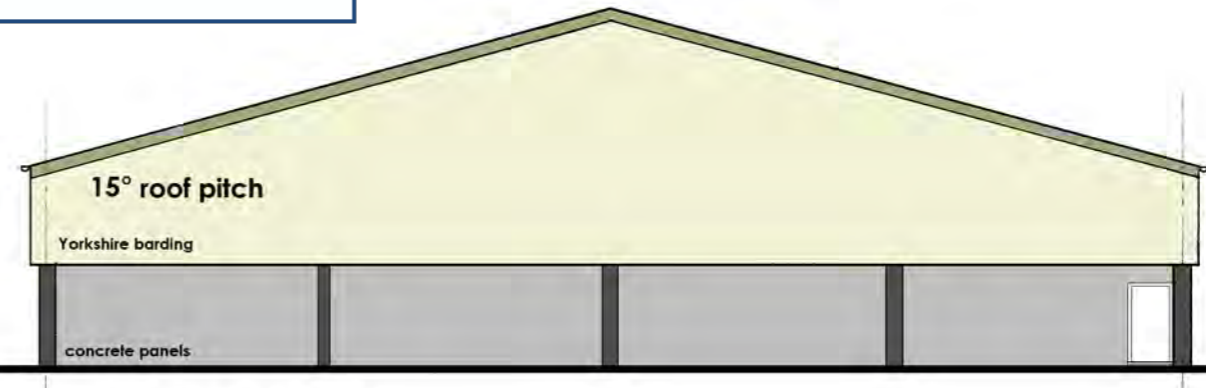
SOUTH ELEVATION
