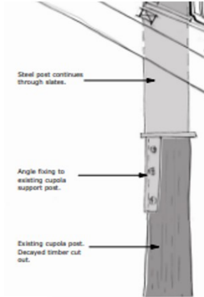
Approved Drawing showing steel angle and photo showing typical installation
