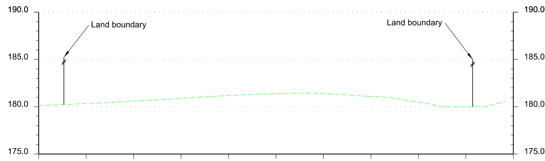
Section B-B Scale H 1:500 V 1:250
