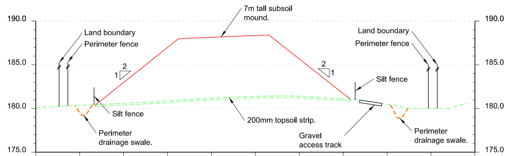
Section B-B Scale H 1:500 V 1:250
