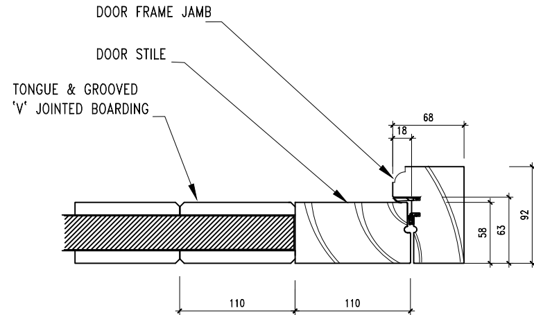
SECTION C 1:5
