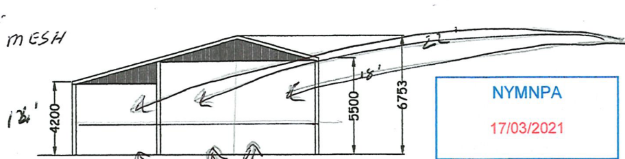
North Elevation 15' METAL GATES
