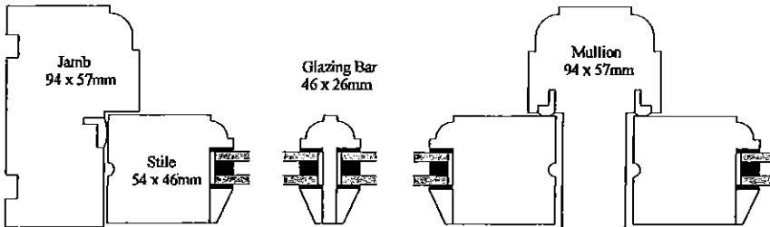
Section through Jamb, Mullion, Sash Stiles & Glazing Bar
