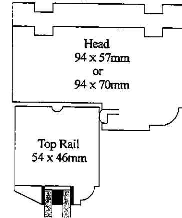
Section through Sill, Head Sash Top & Bottom Rails & Glazing Bar
