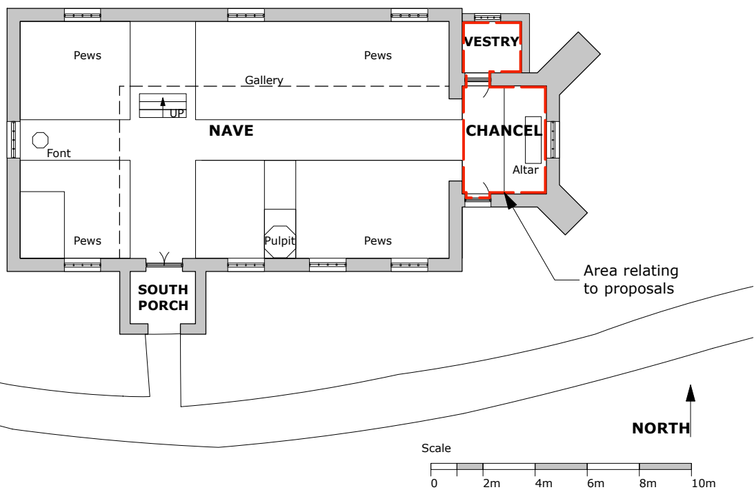
OLD ST STEPHENS CHURCH Indicative plan - existing Approx. scale 1:200
