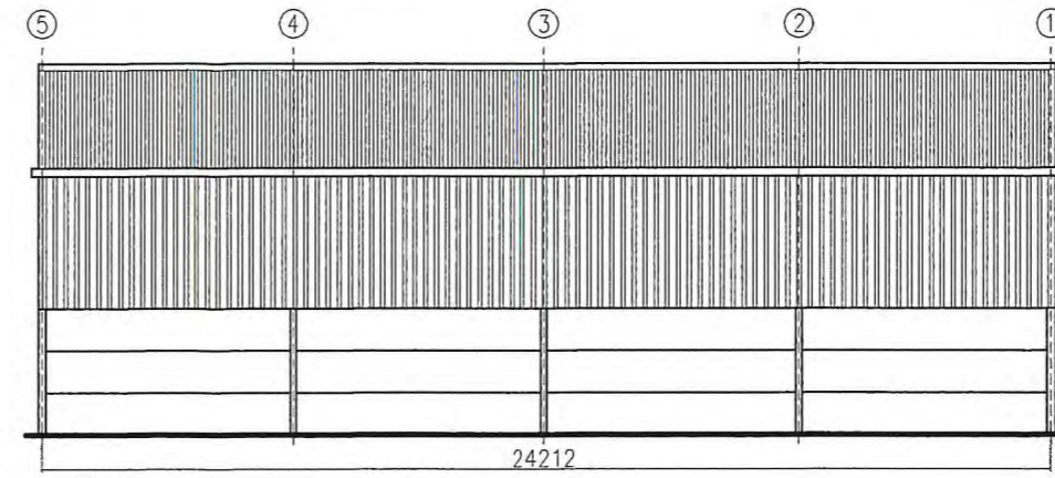
South View 1:200
