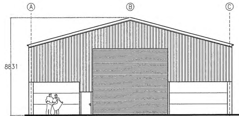
East View 1:200
