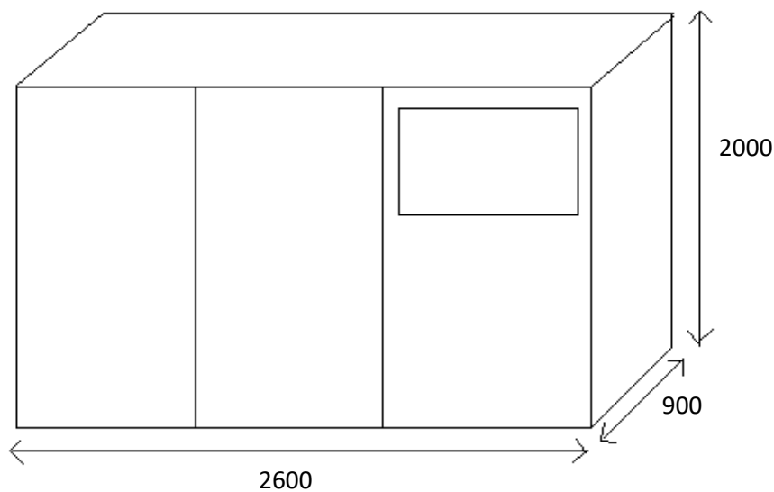
Figure 5a. Bell tent bathroom unit dimensions
