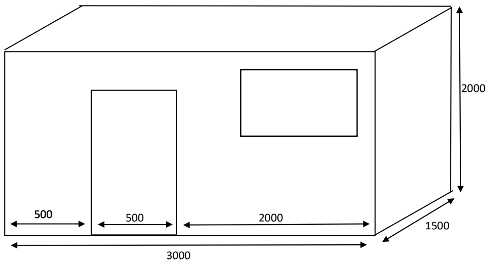
Figure 5. Composting toilet
