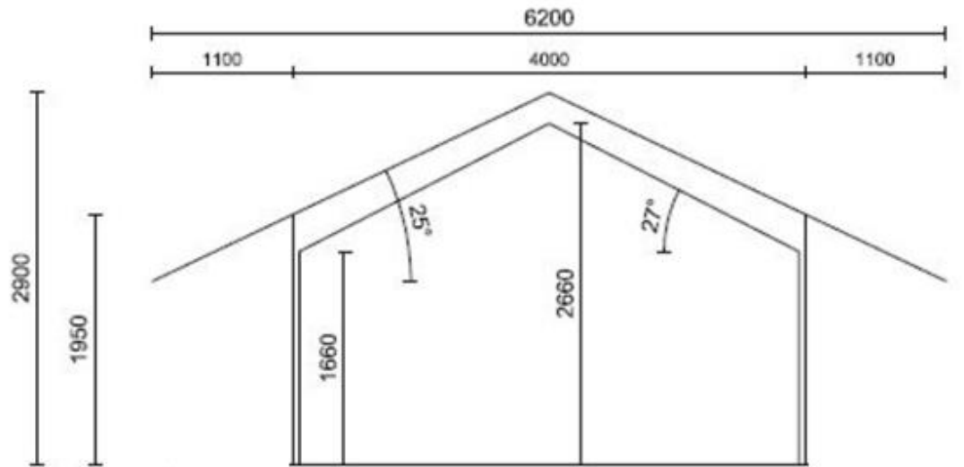
Figure 2a and 2b. Safari tent dimensions
