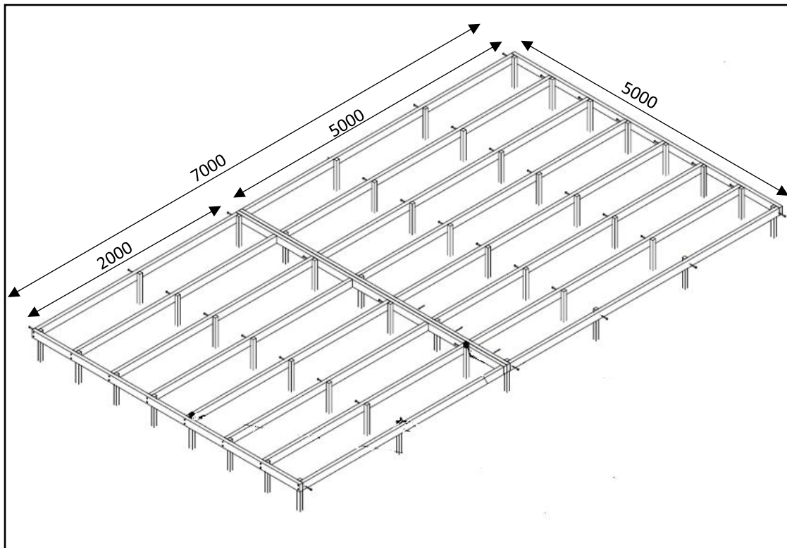
Figure 3. Bell tent base
