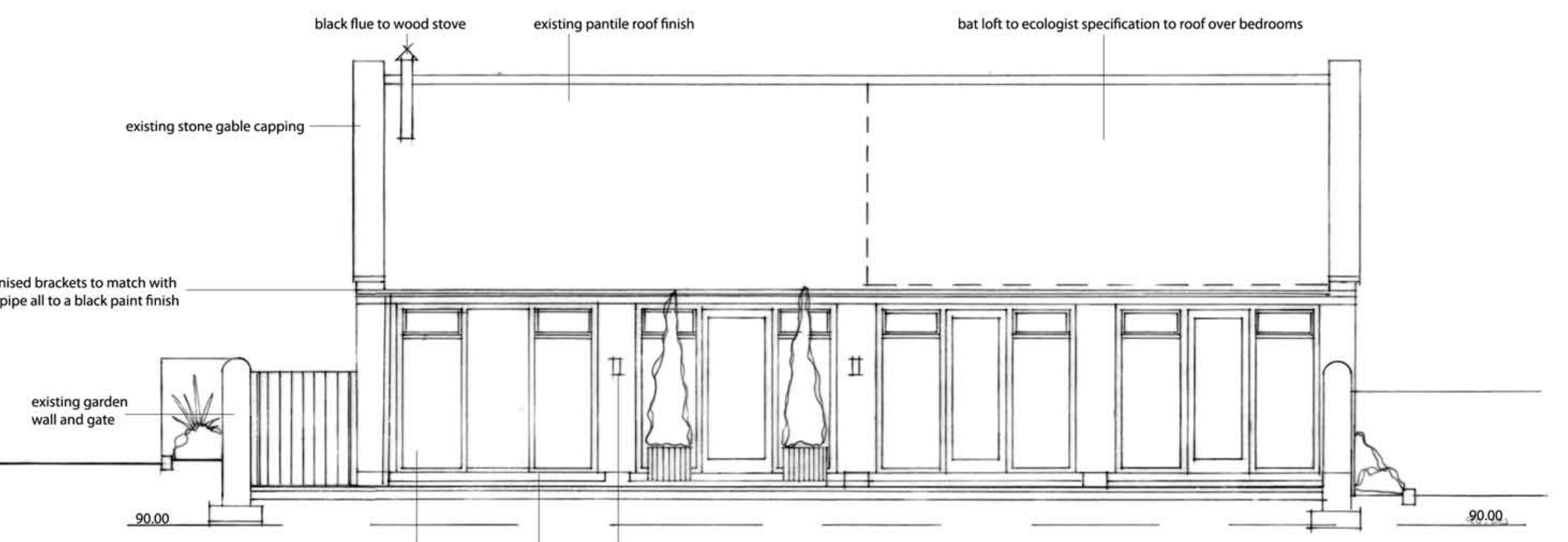
North Elevation
