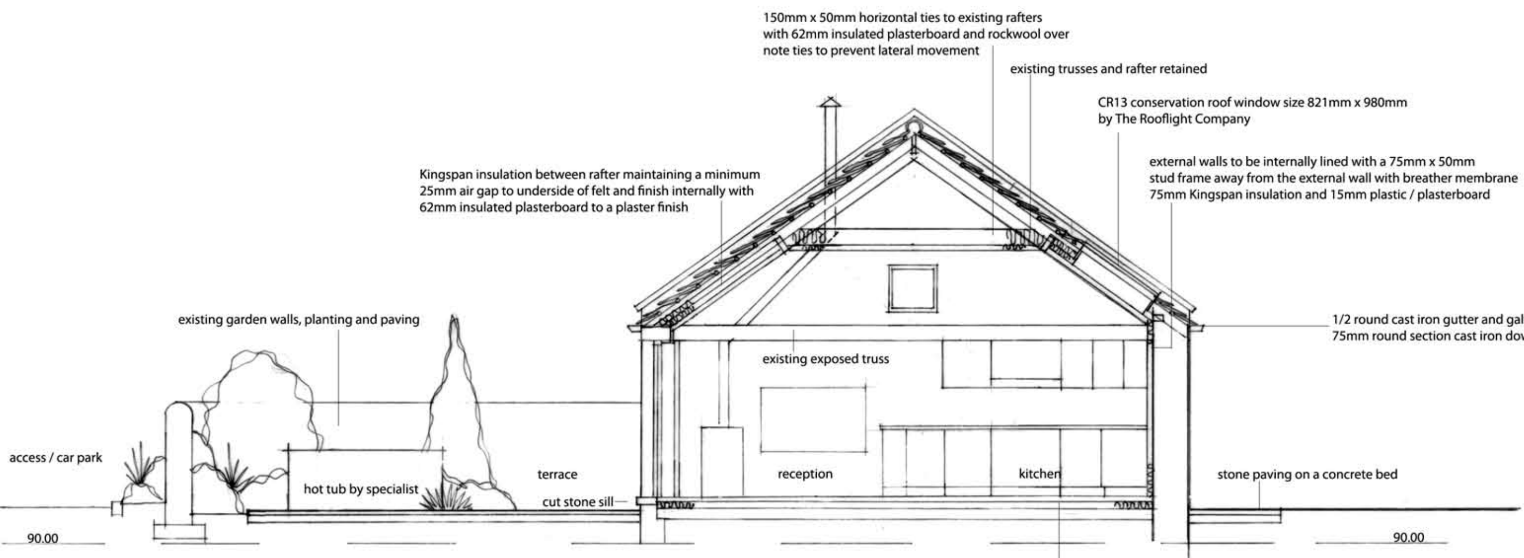
Typical Section
