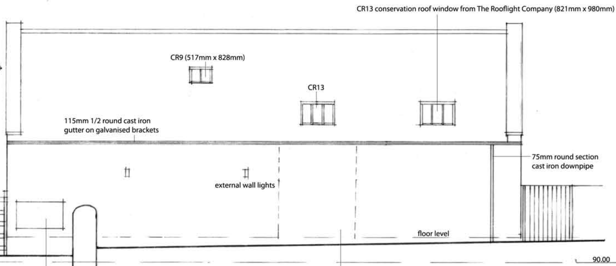
South Elevation
