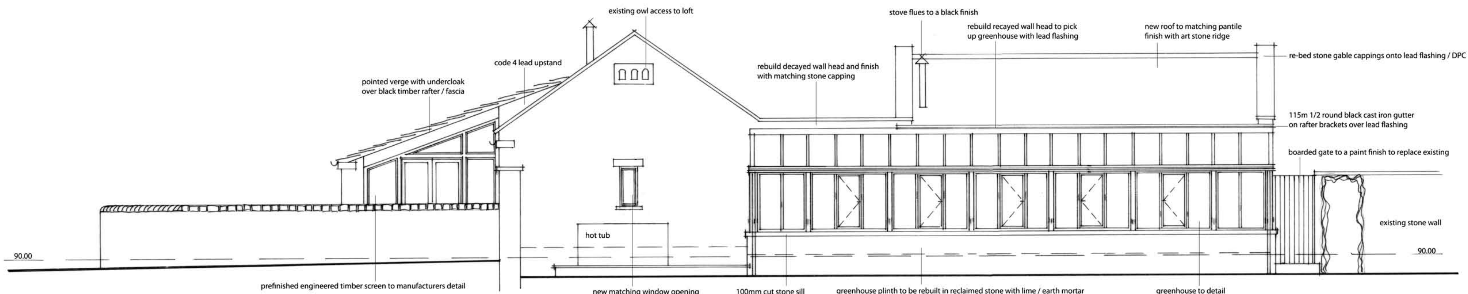
South Elevation
