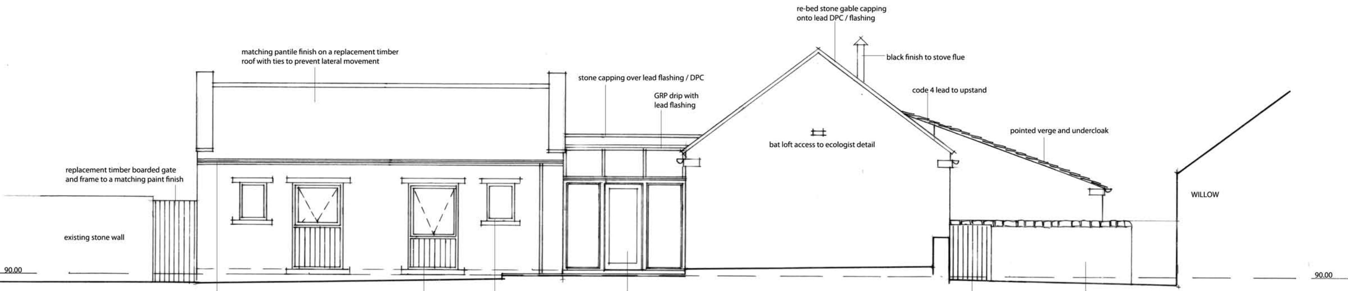
North Elevation
