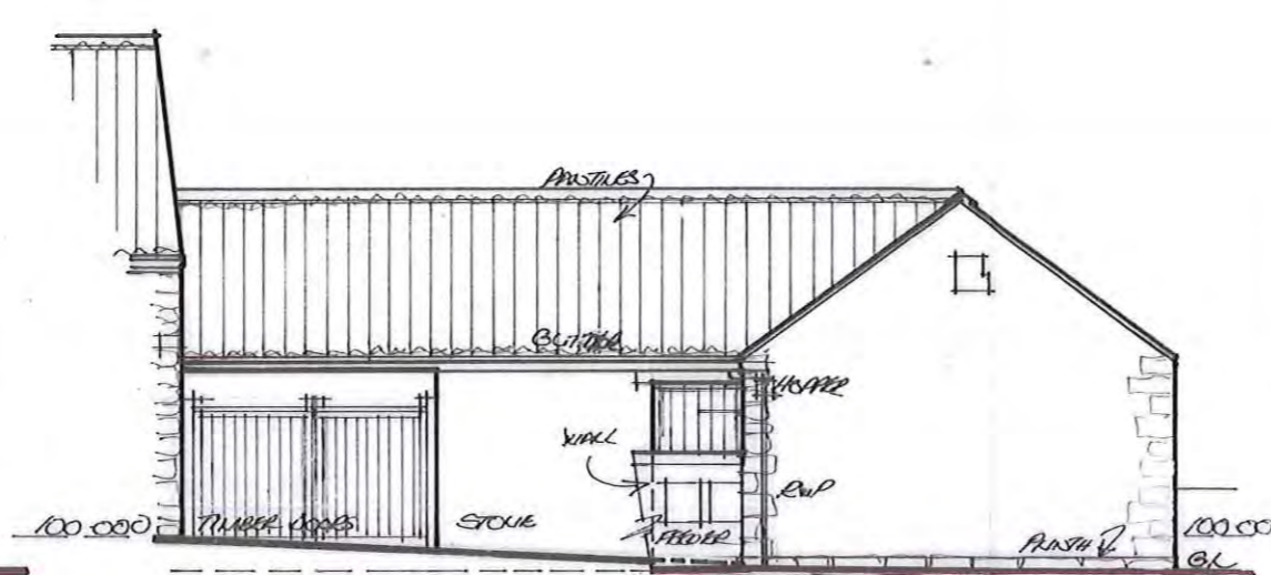
SOUTH ELEVATION
