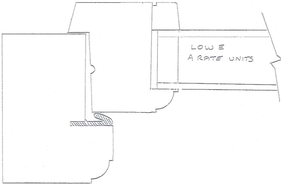
WINDOW AND SASH SECTION |:
