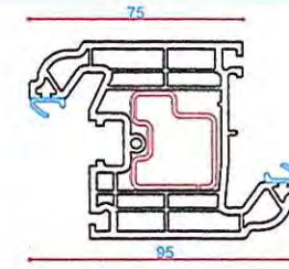
P10545 95mm Z Tran/Slim Open In Door Sash Steel Box S00158
