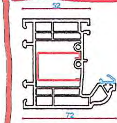
P10532 72mm Outer Frame Steel U Channel S00186 Thermal insert P10332
