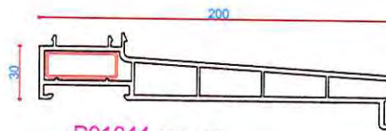
P01044 200mm Cill End Caps M00033 Steel 40 x 15 S00016
