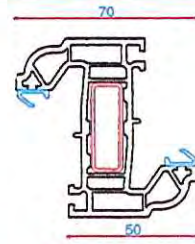
P10536 70mm Z Transom Steel Box S00187
