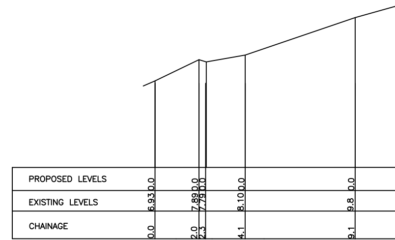
Cross Section D-D
