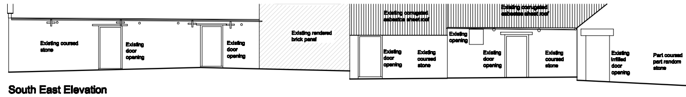
South East Elevation
