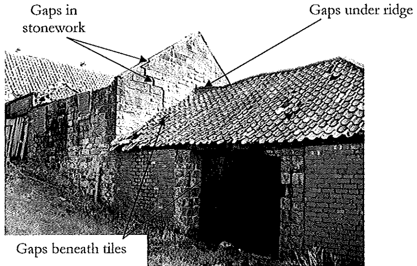
Figure 2 – East elevation.
