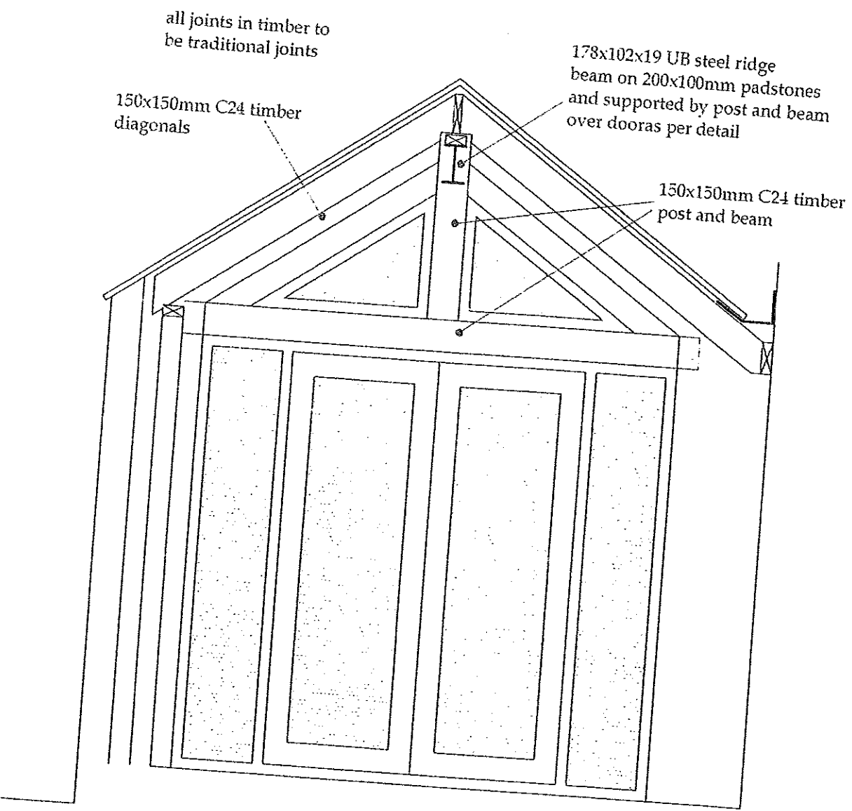
OPTION 1: ridge beam
