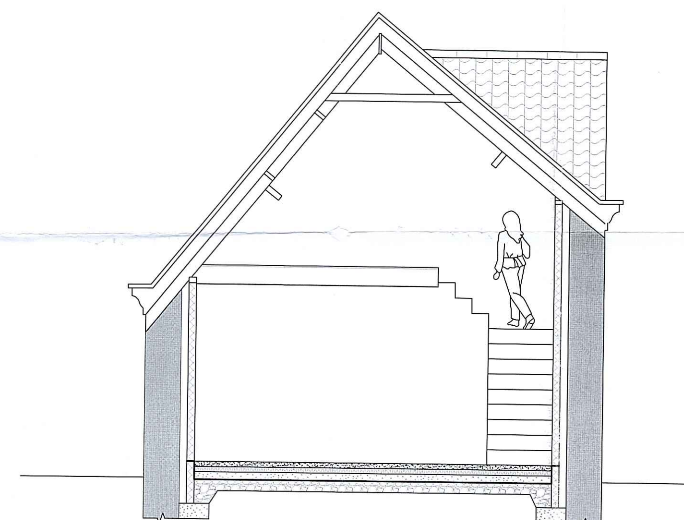
TYPICAL SECTION
