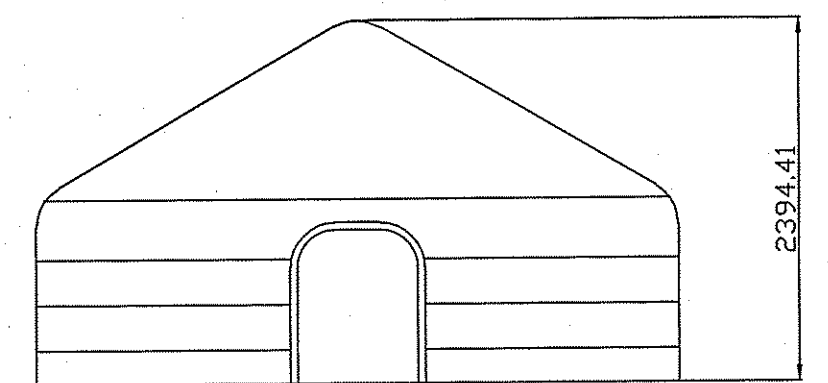
YURT ELEVATION
