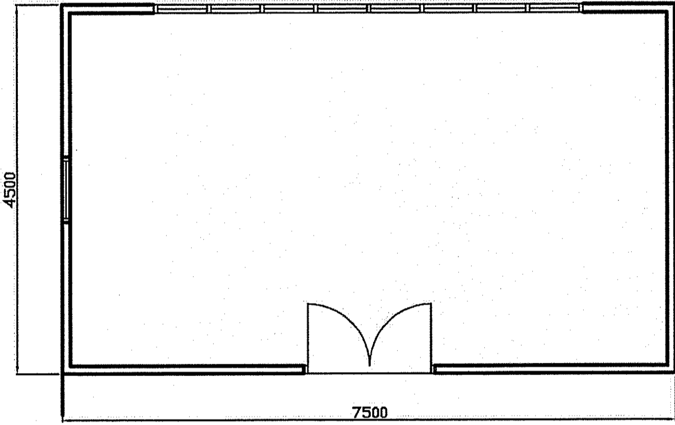
SHED PLAN
