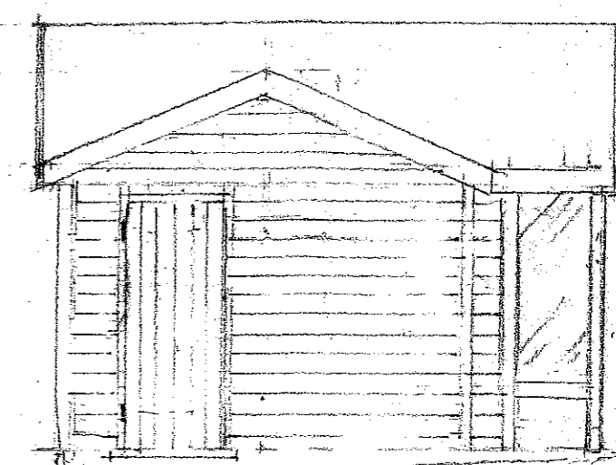
LEFT SIDE ELEVATION 4000
