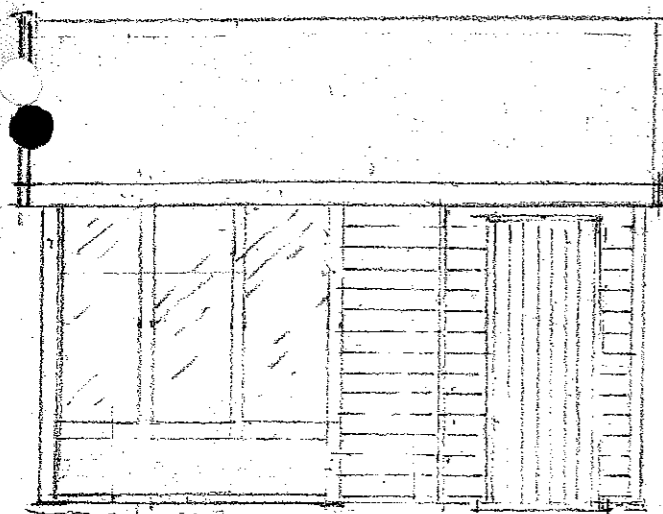
RIGHT SIDE ELEVATION 4000
