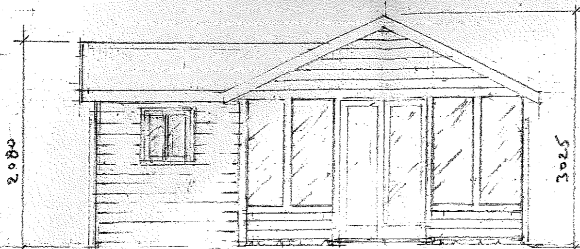
FRONT ELEVATION 6000
