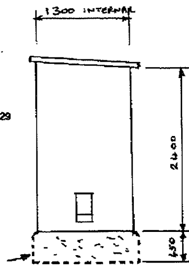
WEST ELEVATION
