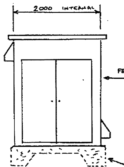
NORTH ELEVATION
