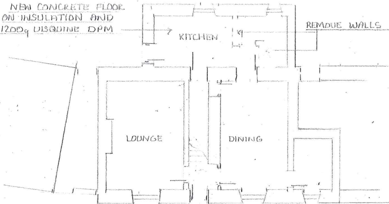
GROUND FLOOR
