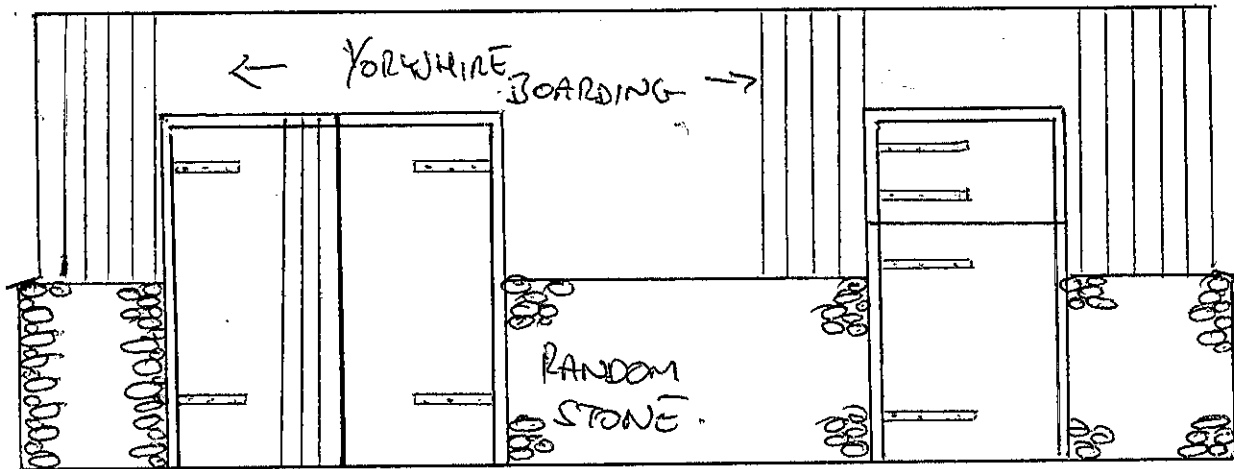
LEDGED AND BRACED DOUBLE GARAGE DOORS.
