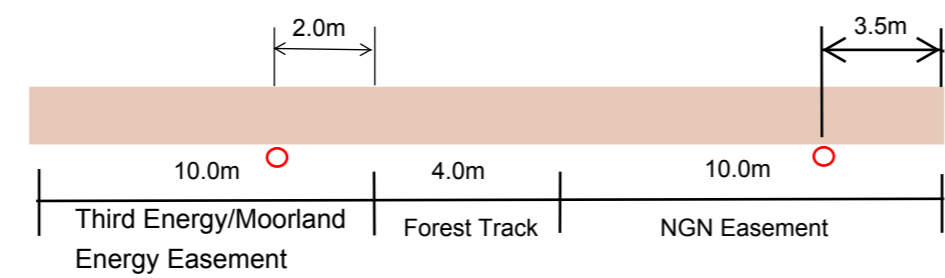
DALBY FOREST TRACK EASEMENT CONFIGURATION
