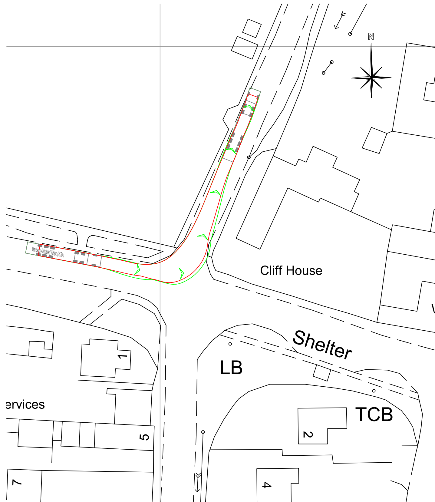
Swept Paths at Eberston A170 Junction
