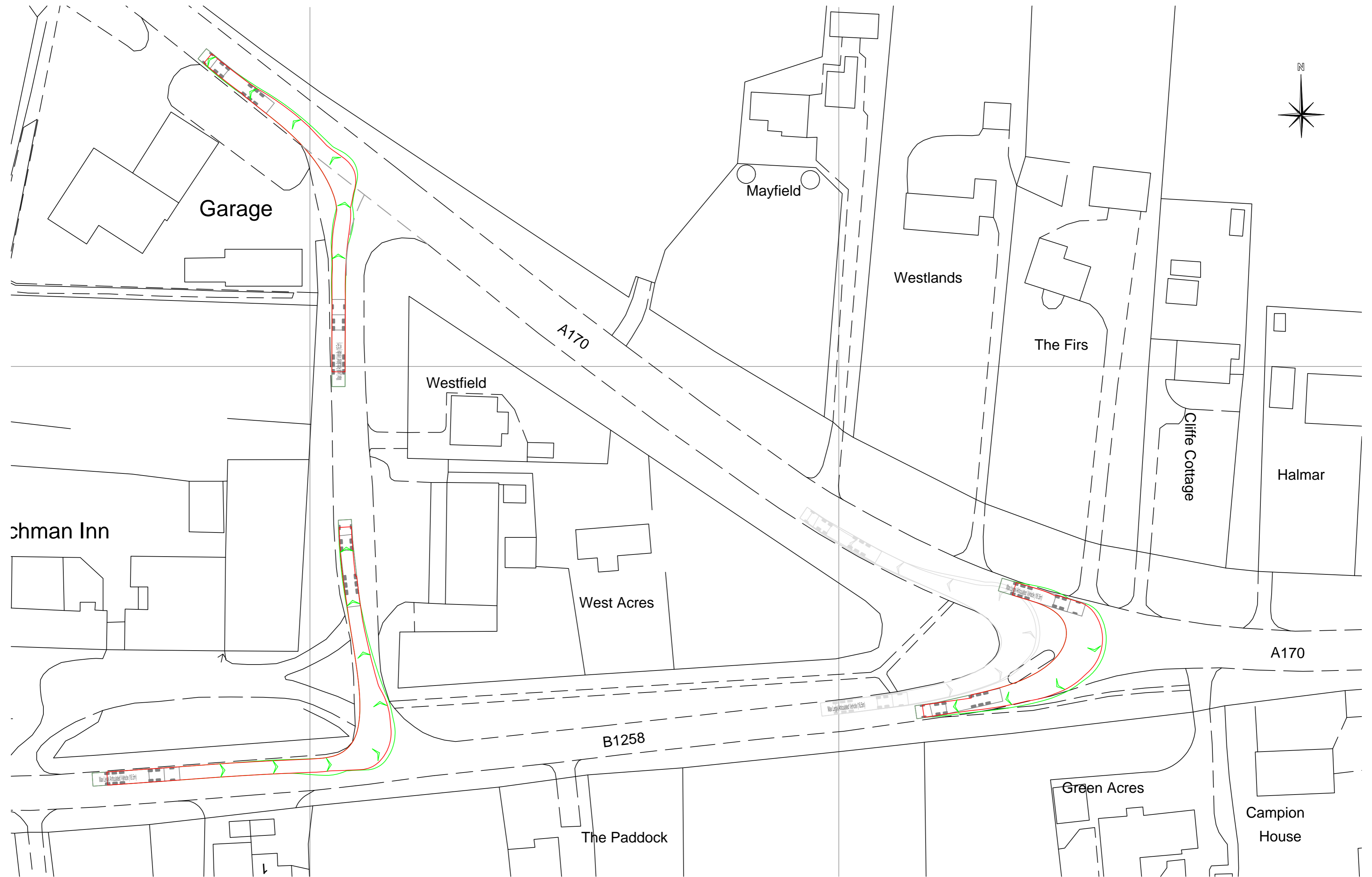
Swept Paths at Snainton A170 Junction
