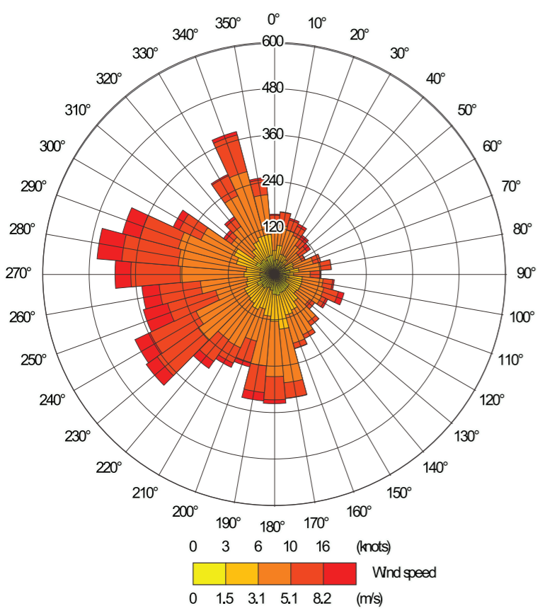
Church Fenton Wind Rose for 2012
