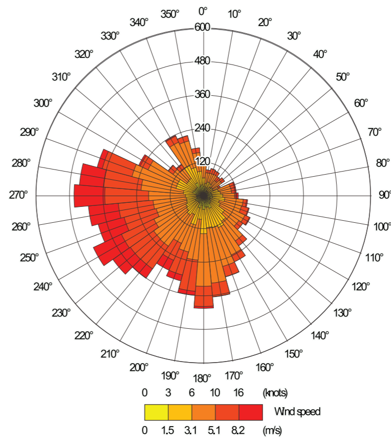
Church Fenton Wind Rose for 2011
