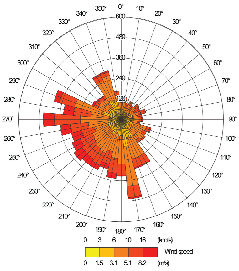
Church Fenton Wind Rose for 2009
