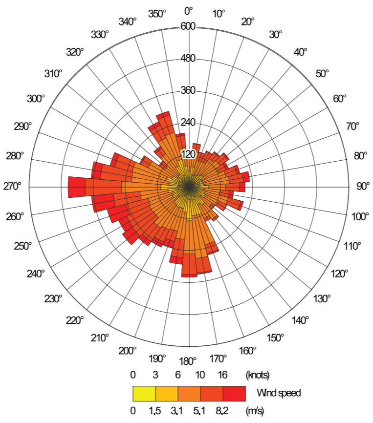
Church Fenton Wind Rose for 2013
