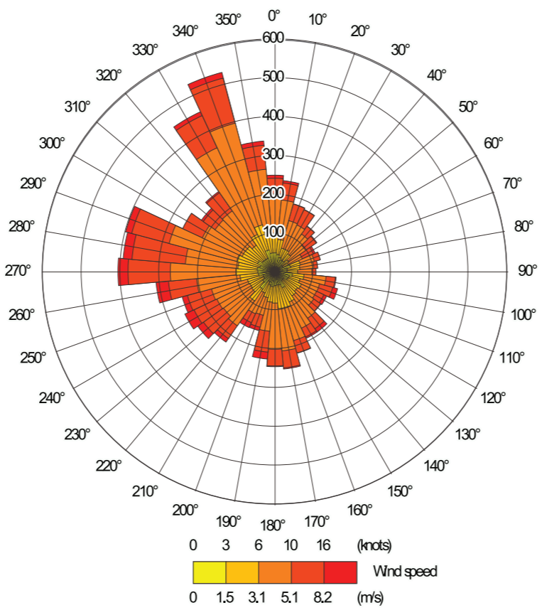
Church Fenton Wind Rose for 2010
