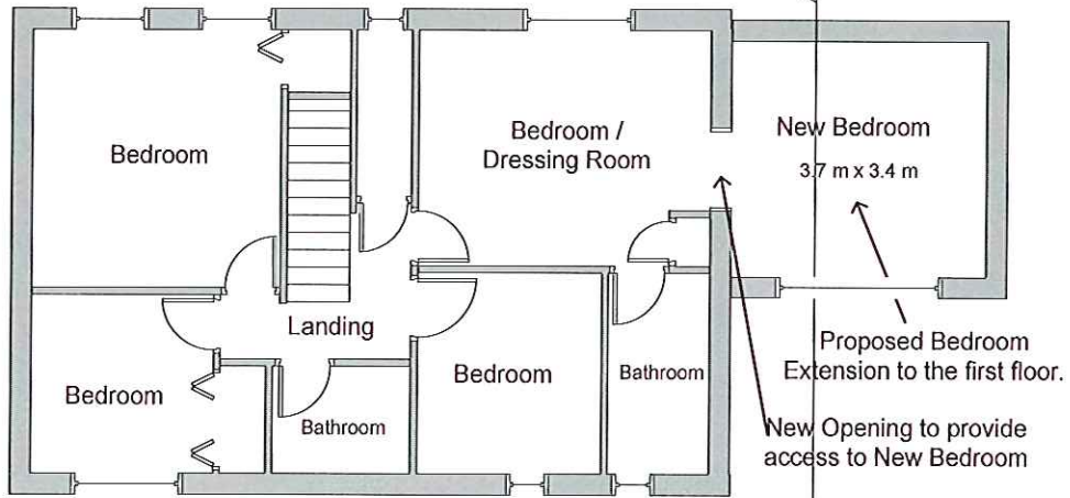
First Floor Layout showing proposed New Bedroom
