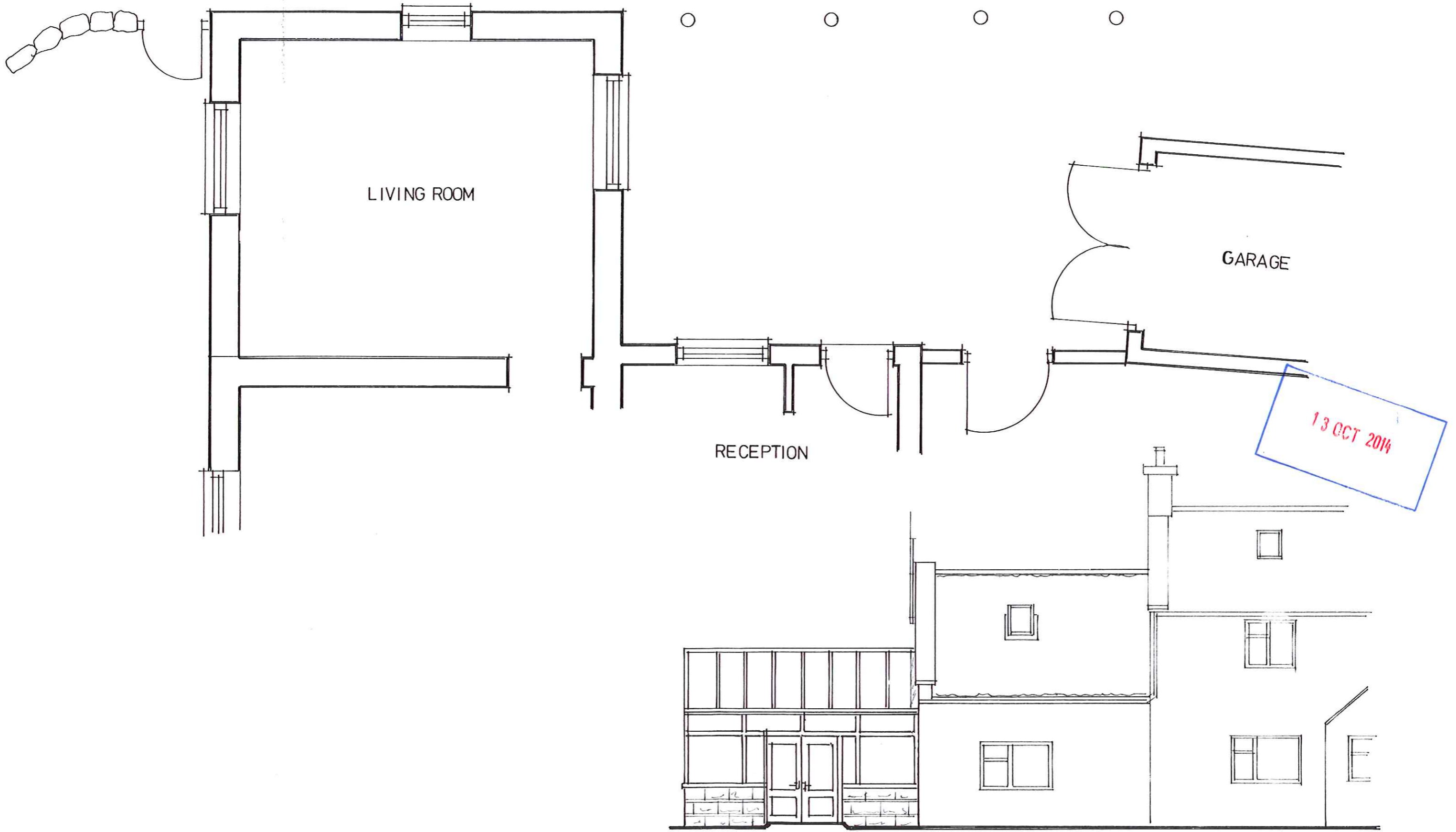
PROPOSED CONSERVATORY TO ROSE COTTAGE, FORMING RECEPTION TO HIGHGATE HOWE HOLIDAY HOME PARK, WHITBY for Mrs L TROTTER PLAN AS EXISTING AND PROPOSED ELEVATION
