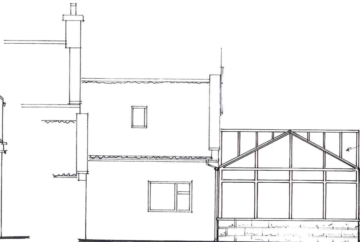
WEST PROPOSED
