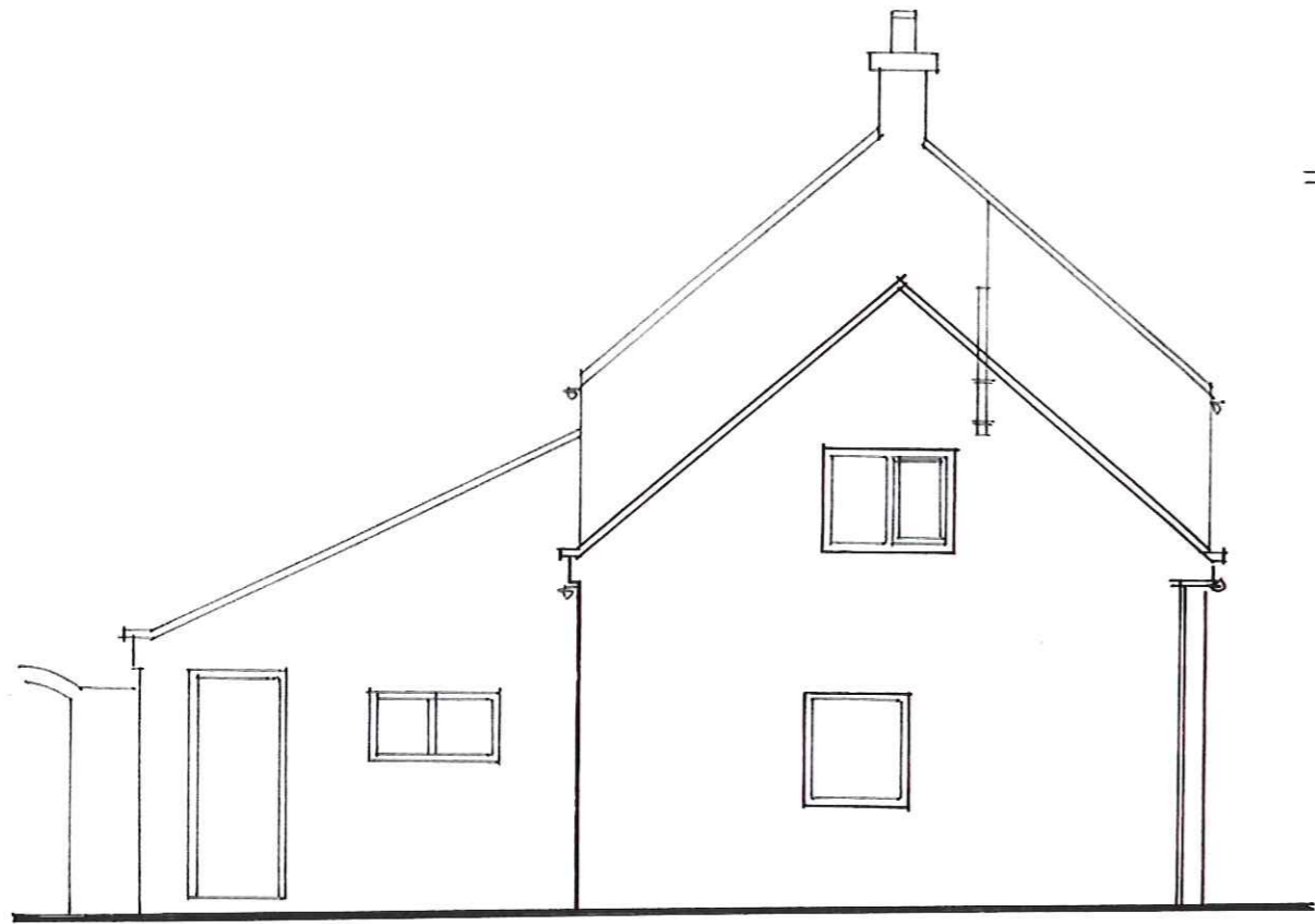
SOUTH EXISTING
