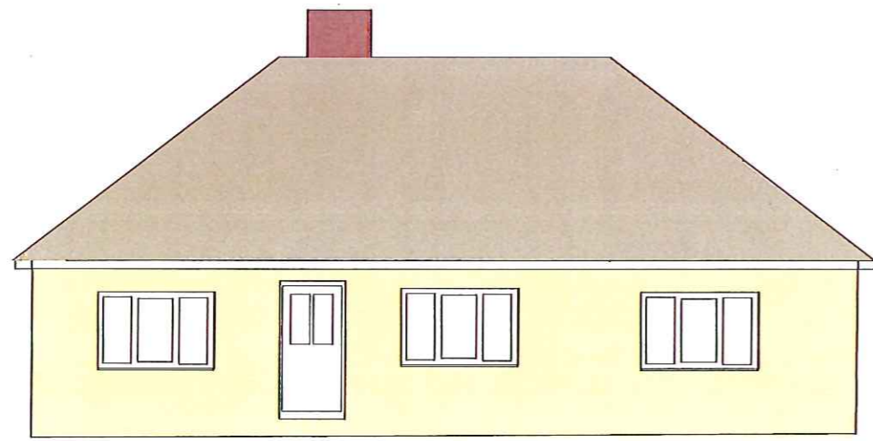
East Elevation Existing
