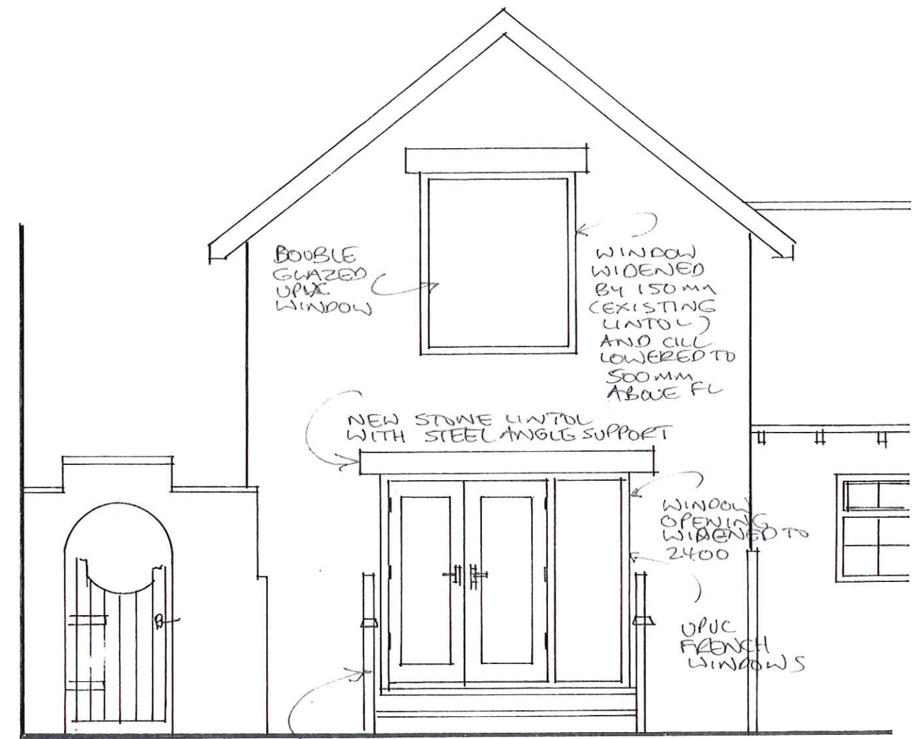
WEST ELEVATION PROPOSED
