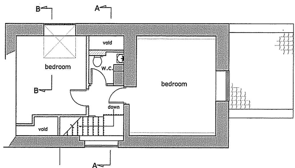
FIRST FLOOR LAYOUT
