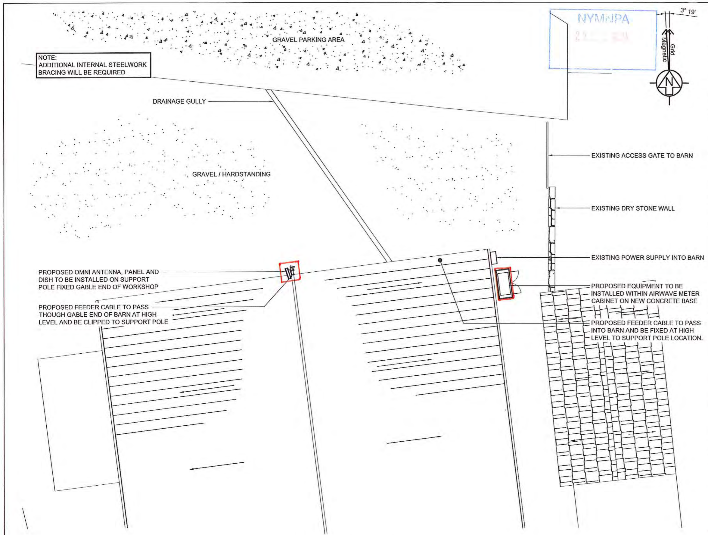
PROPOSED SITE PLAN (SCALE 1:100)
