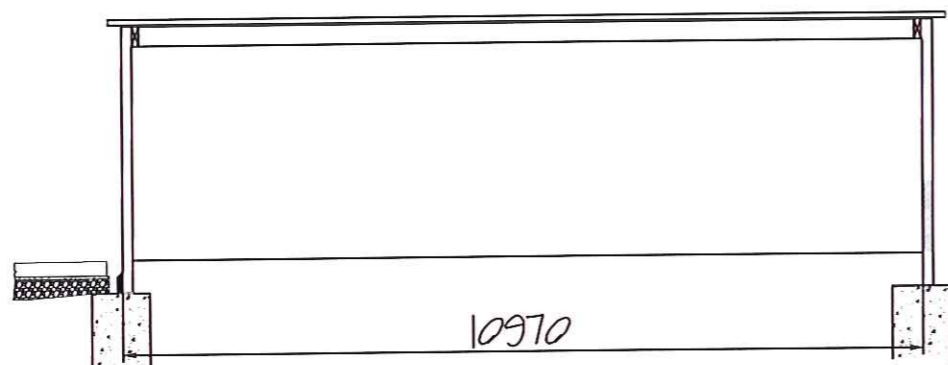
LONG SECTION
