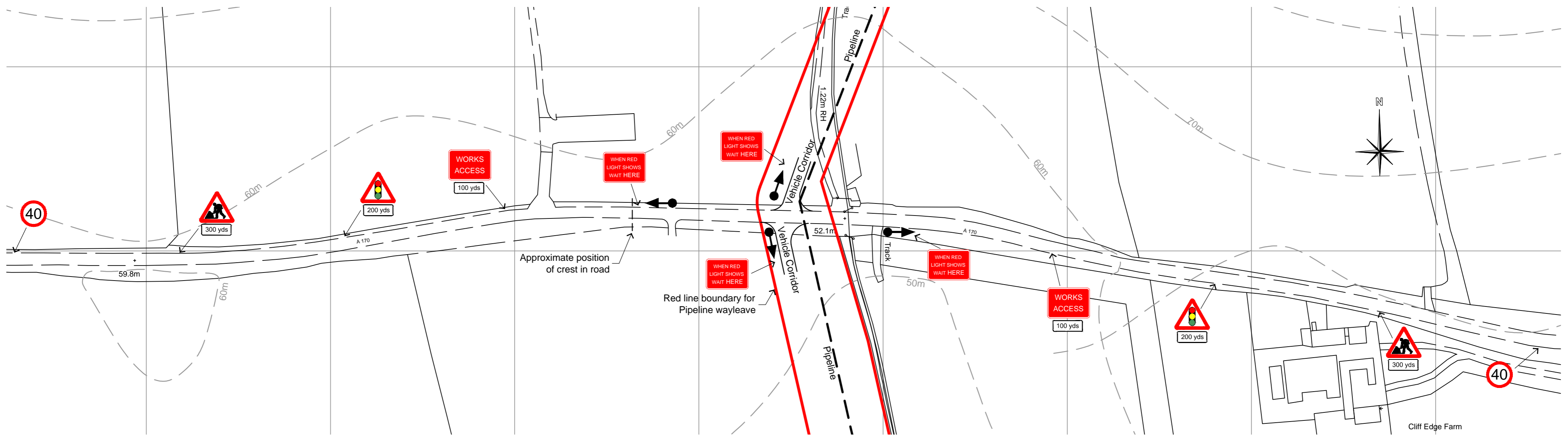
Proposed Traffic Control at Site Crossing of A170
